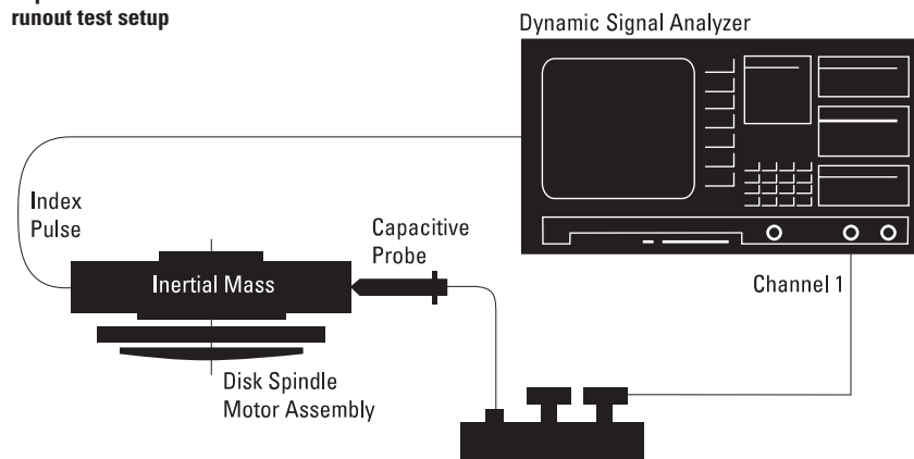
Figure 1: Experimental runout test setup
