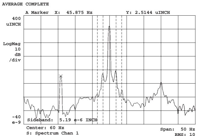
Figure 8: A zoom measurement at 60 Hz shows sidebands spaced 2.5 Hz, an indication of precession.
